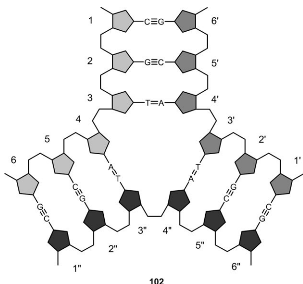
Figure 3. DNA-junction showing the DNA sequence 5'-d(CGTCAG)-3' and the base-pair arrangement.
