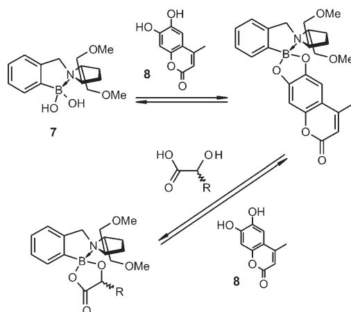
Scheme 1. Enantioselective displacement assays for the fluorescent indicator 4-methylesculetin.
