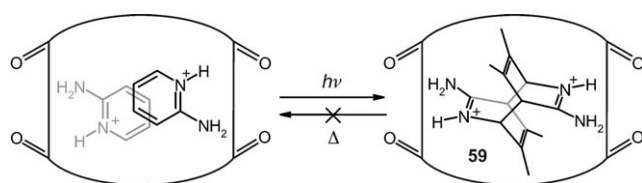
Scheme 5. Photodimerization within cucurbit[7]uril.
