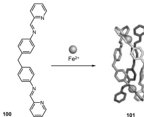
Scheme 12. Formation of metallocsupramolecular triple helicate 101 .
